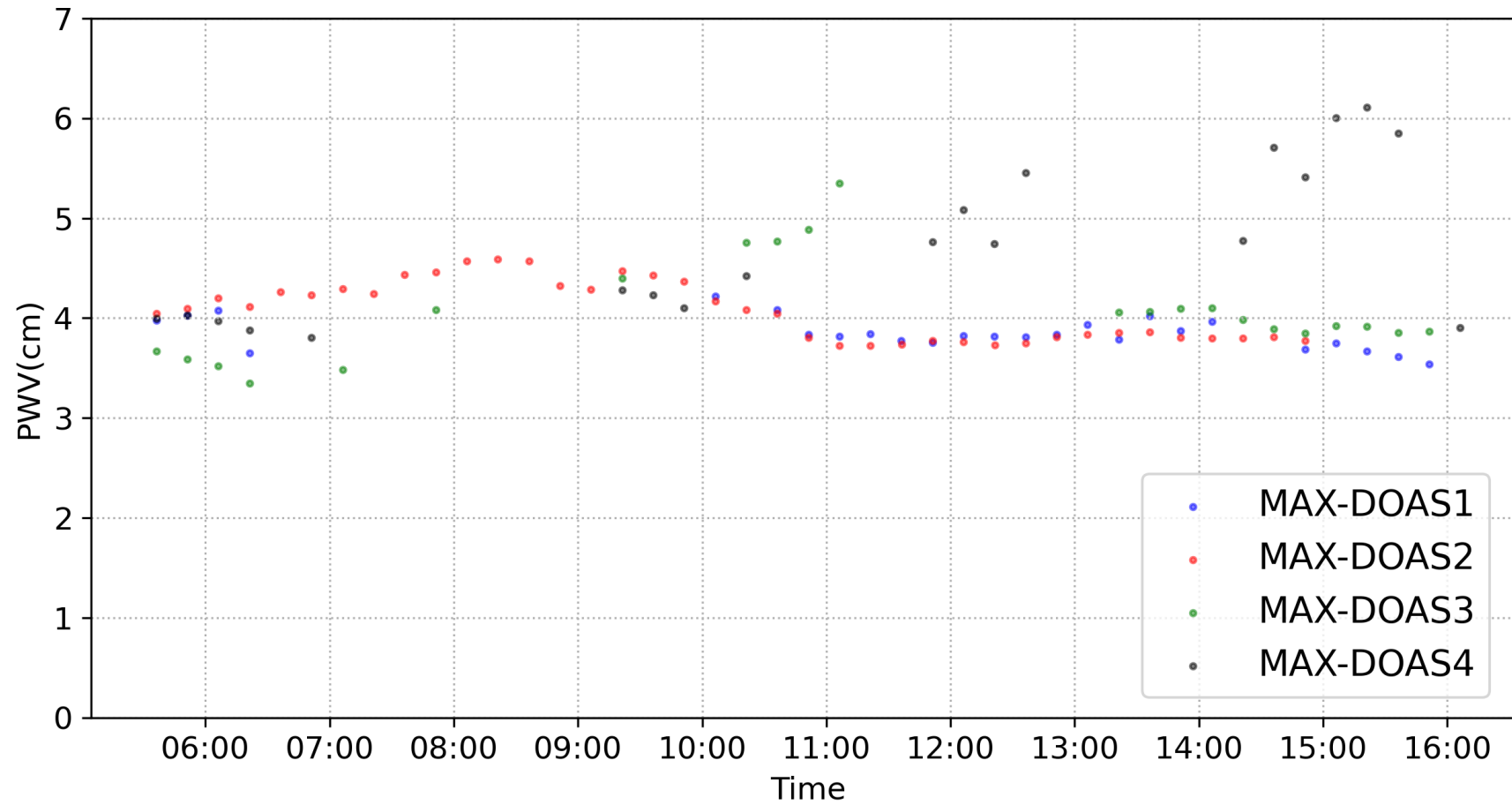
PWV(cm) of MAXDOAS1-4 in Chiba 2021/08/04
